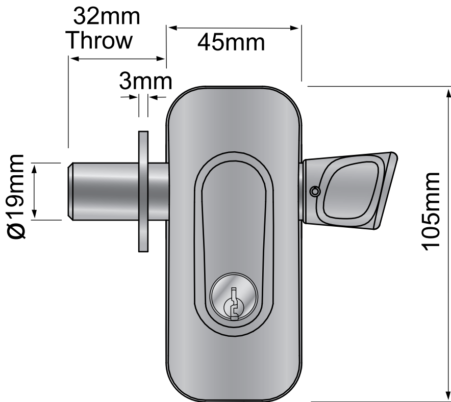
SIDE MOUNT MODEL
