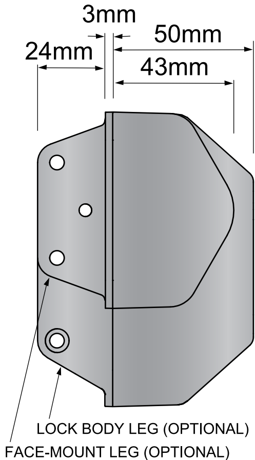
FACE-MOUNT MODEL
