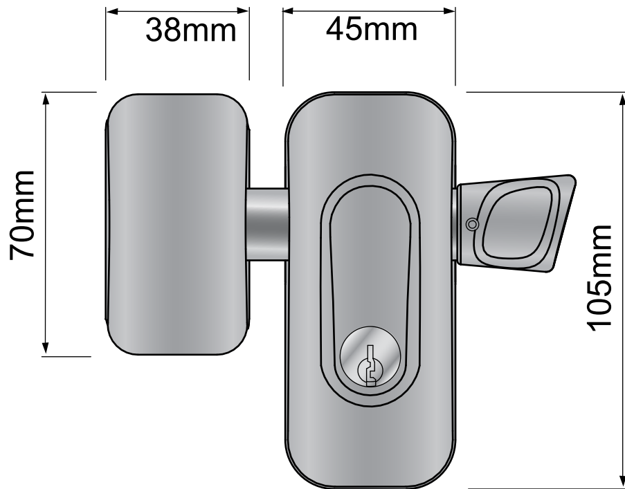
FACE-MOUNT MODEL
